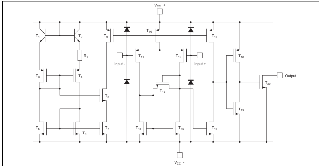
Figure 1. Schematic diagram (for one channel of JTS393)
